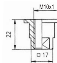
Dimensions of coupling
