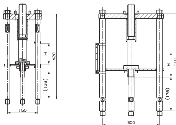
Attachment yoke DN 200 - 400 Attachment yoke DN 600 Output drive type A, F10, Tr36x6-LH Output drive type A, F10, Tr36x6-LH
