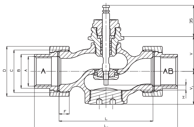
Valves RV 111 S/T with threaded connection
